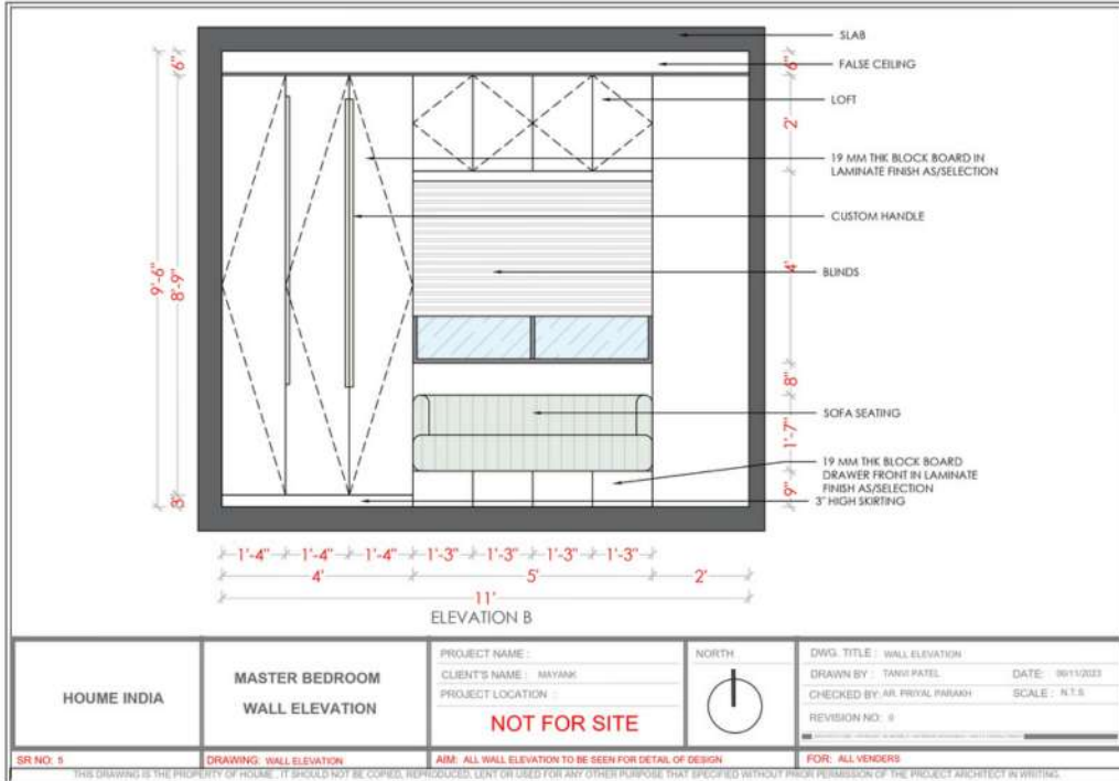
Elevation of the Wardrobe - Best for Appartments
